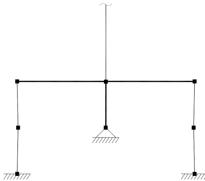
Fig. 6.18 Analytical model of \mu NEES specimen.
