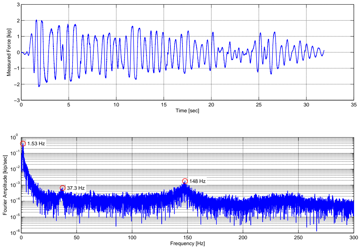
Fig. 6.14 Measured force history and Fourier amplitude spectrum from STS.
