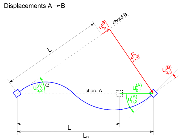
Fig. 3.17 Nonlinear transformation from basic system A to B.
