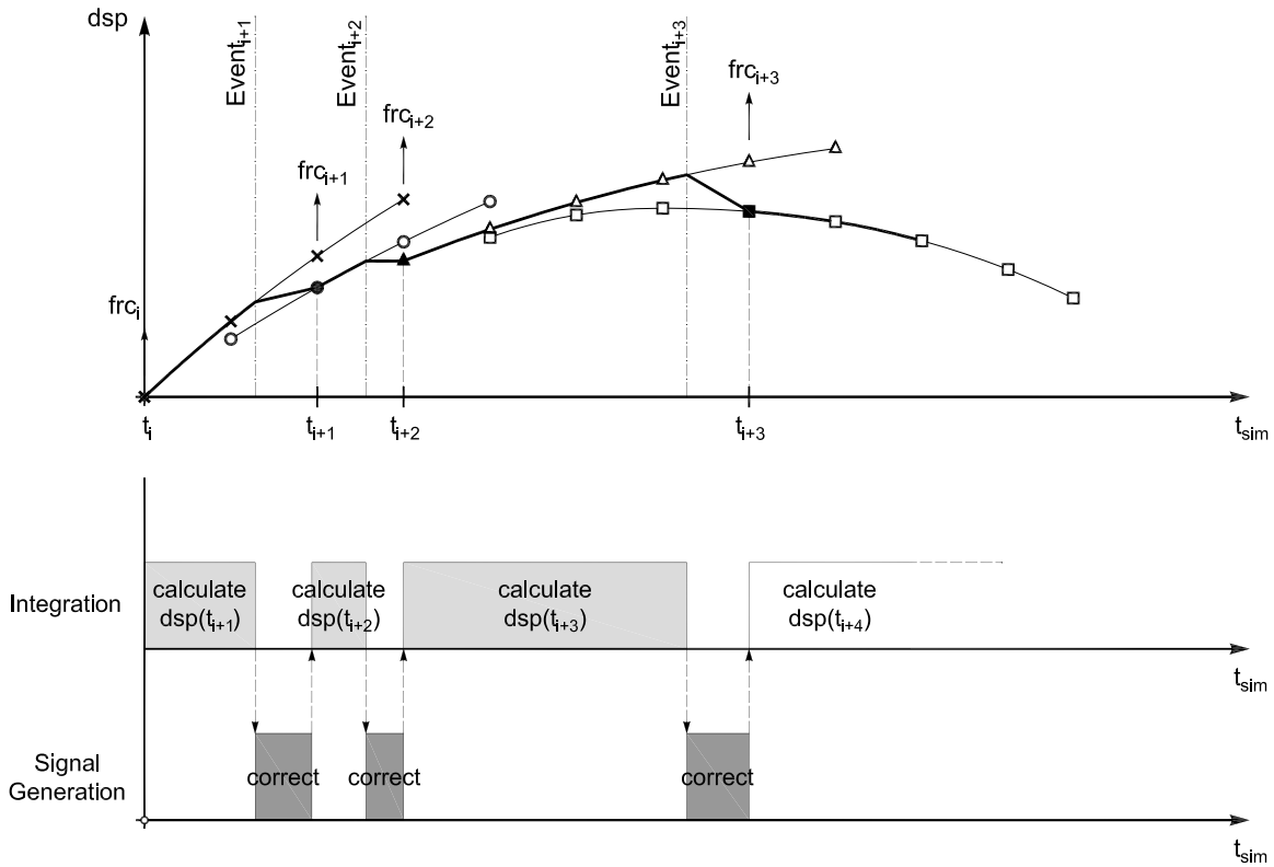
Fig. 5.21 Displacement path and execution sequence of first adaptive integration time-step strategy.
