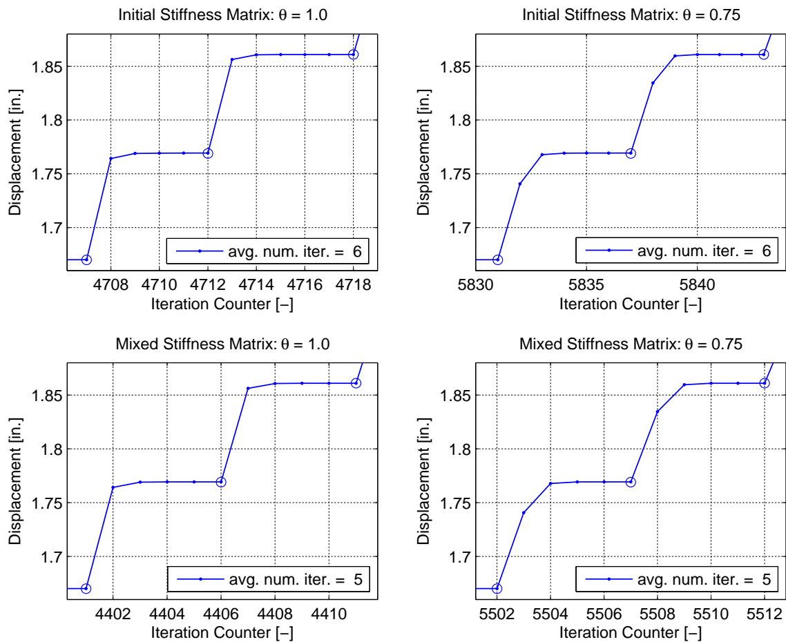
Fig. 4.7 Krylov-Newton convergence comparison for four-story-frame model.
