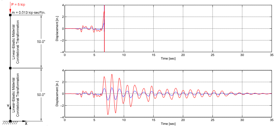
Fig. 4.21 Cantilever column response for linear-elastic material behavior and nonlinear, corotational transformation: (a) model, (b) G\alpha OS1 , (c) G\alpha OS2 .
