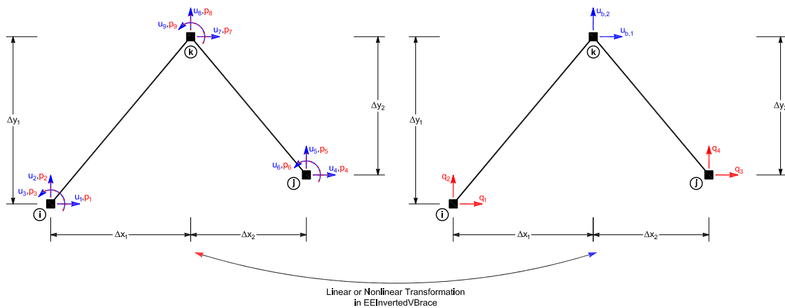
Fig. 3.21 Experimental inverted-V brace element (EEInvertedVBrace2d).
