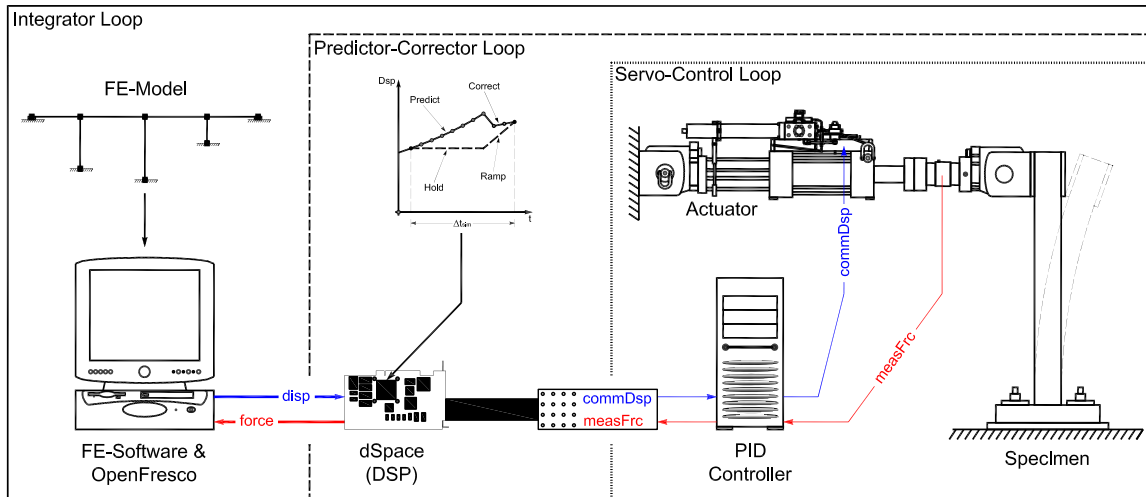
Fig. 3.27 dSpace experimental control (ECdSpace).
