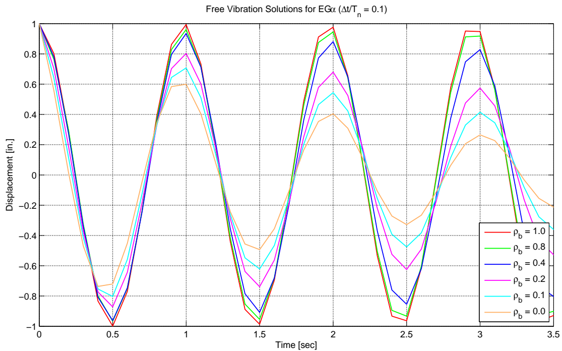
Fig. 4.24 Free vibration solutions for explicit generalized-alpha (EG \alpha ) method.
