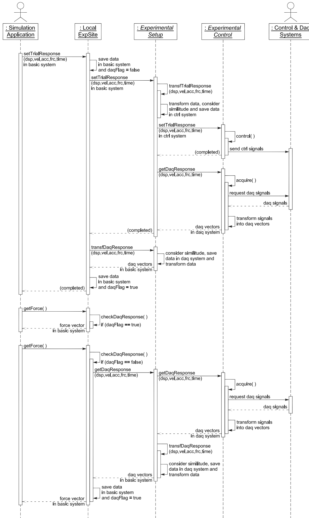
Fig. 3.12 OpenFresco sequence diagram for local deployment.
