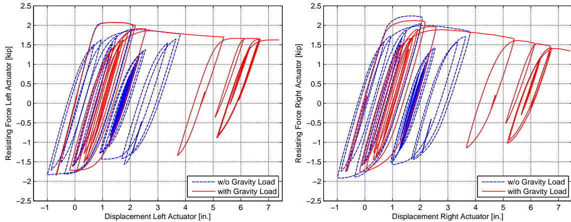
Fig. 6.28 Comparison of actuator force-displacement hysteresis loops for portal-frame model from OpenSees.
