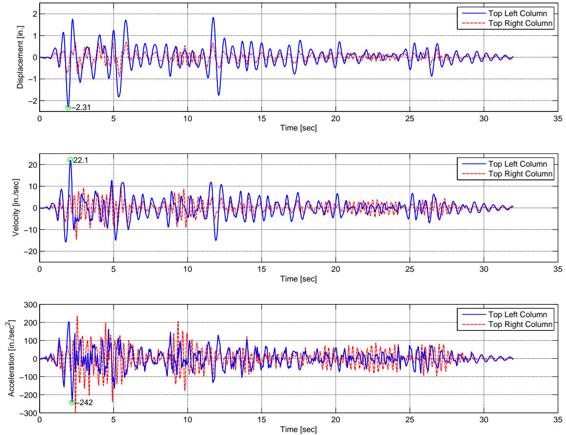
Fig. 6.9 Response histories of one-bay frame model from OpenSees.
