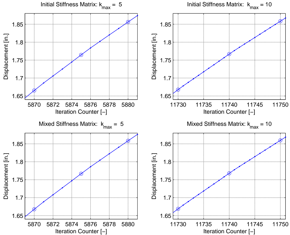
Fig. 4.11 Convergence comparison for four-story-frame model.
