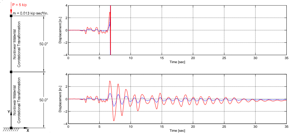
Fig. 4.22 Cantilever column response for nonlinear material behavior and nonlinear, corotational transformation: (a) model, (b) G\alpha OS1 , (c) G\alpha OS2 .
