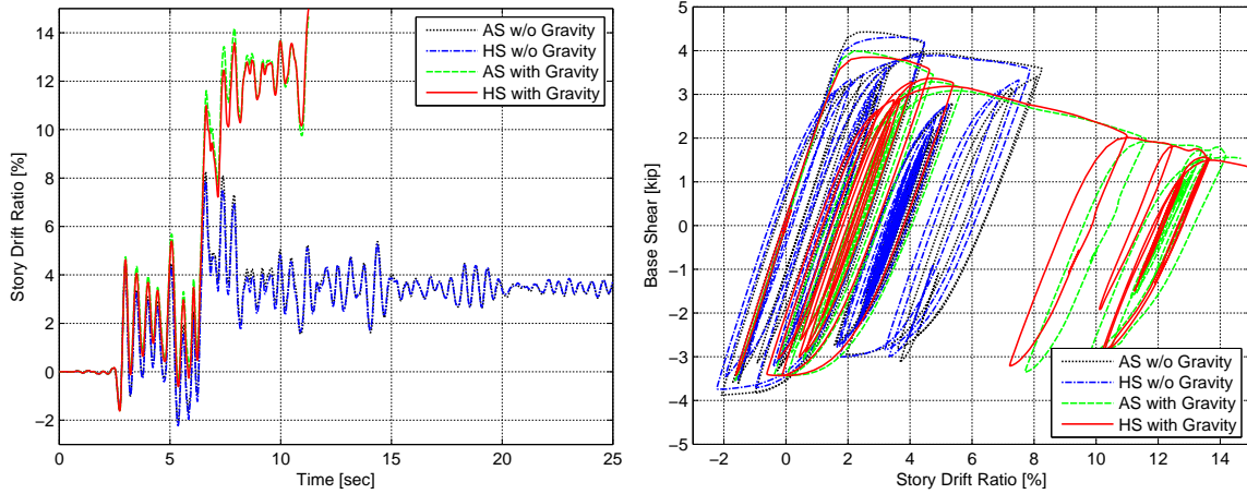
Fig. 6.32 Comparison of story-drift time-histories and total story hysteresis loops of portal-frame model for analytical versus hybrid simulation.
