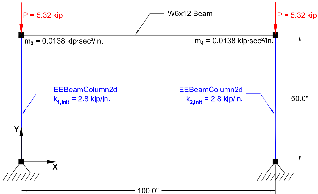
Fig. 6.24 Portal-frame model with structural properties.
