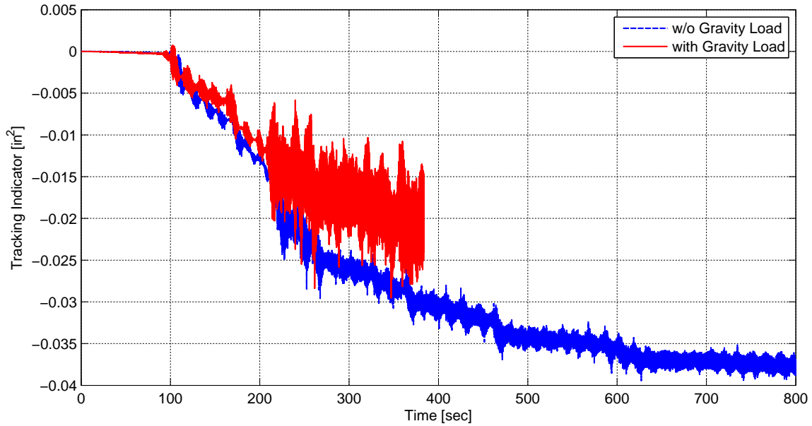
Fig. 6.31 Comparison of tracking performance for test without gravity loads versus test with gravity loads from STS.
