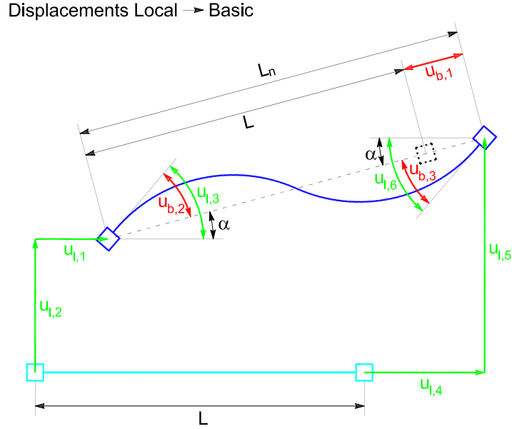
Fig. 6.23 Corotational transformation from local to Basic System A.
