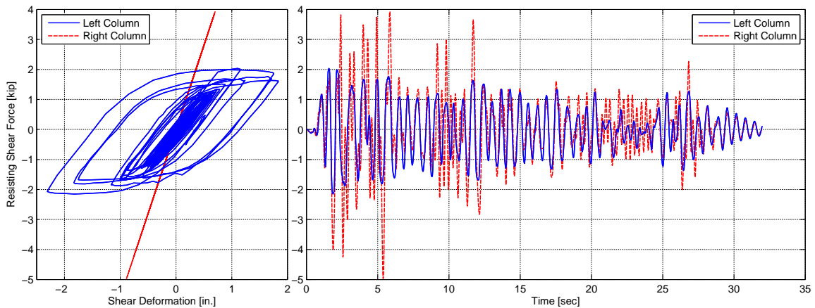
Fig. 6.10 Hysteresis loops and force histories of one-bay frame model from OpenSees.
