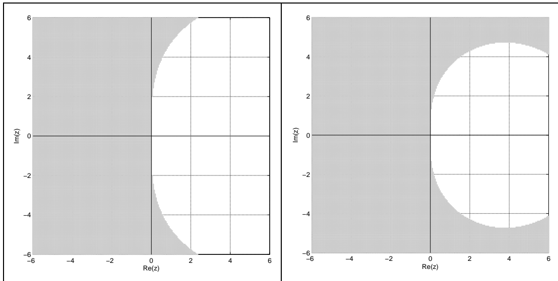
Fig. 4.38 Regions of Absolute Stability (RAS) for RRK methods.
