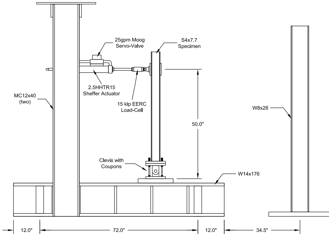
Fig. 6.3 \mu NEES experimental setup with two independent specimens.
