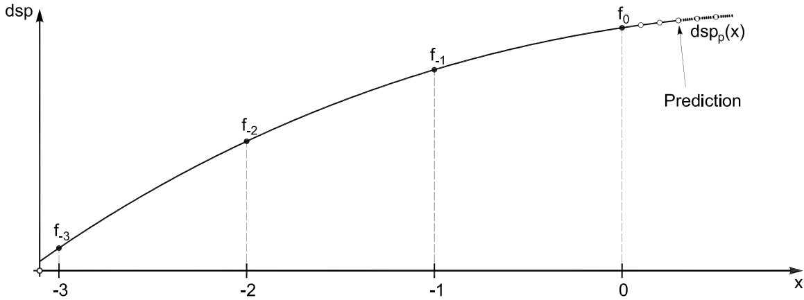
Fig. 5.5 Predictor using a third-order Lagrange polynomial.
