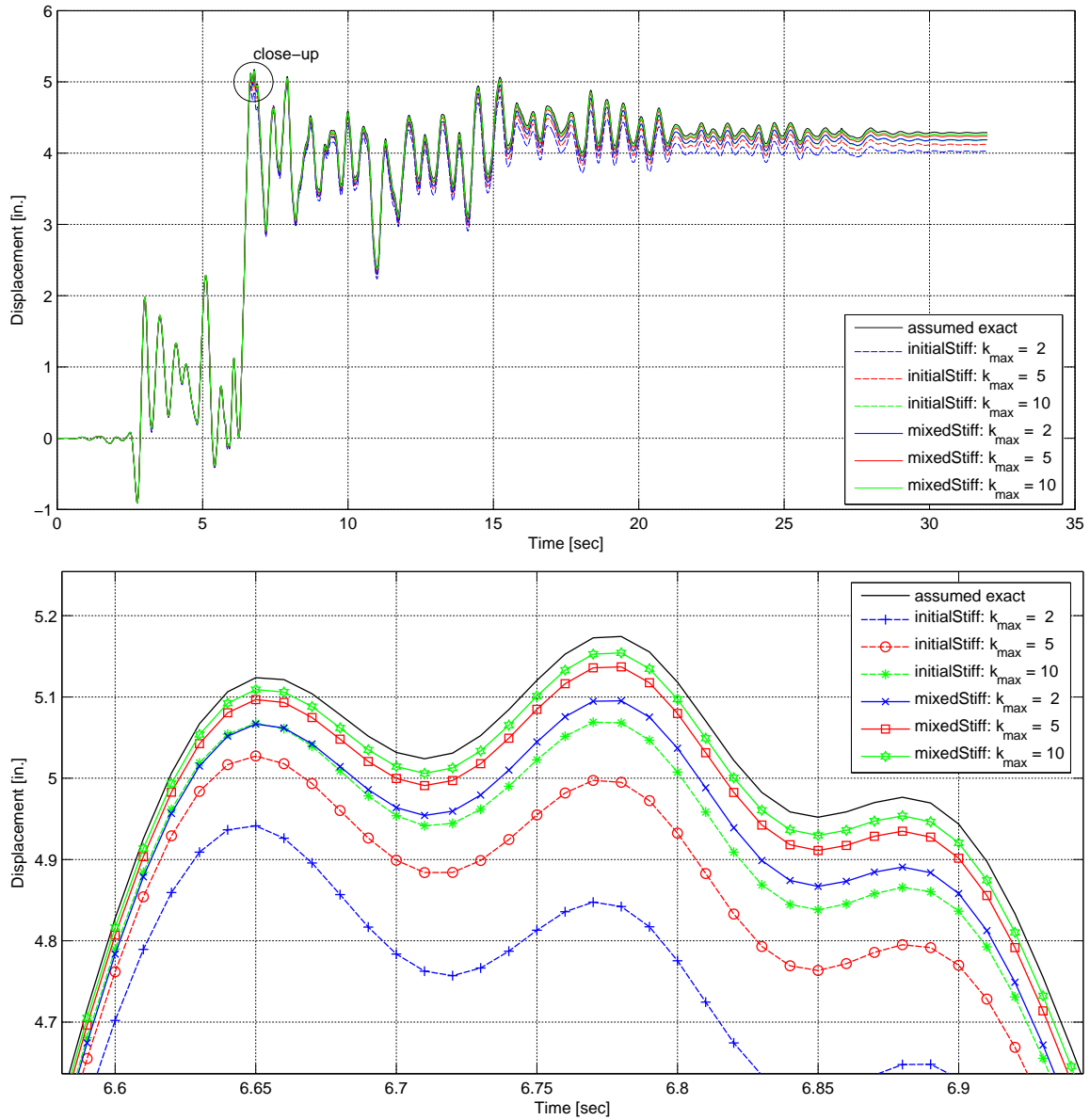
Fig. 4.14 Displacement comparison for portal-frame model.
