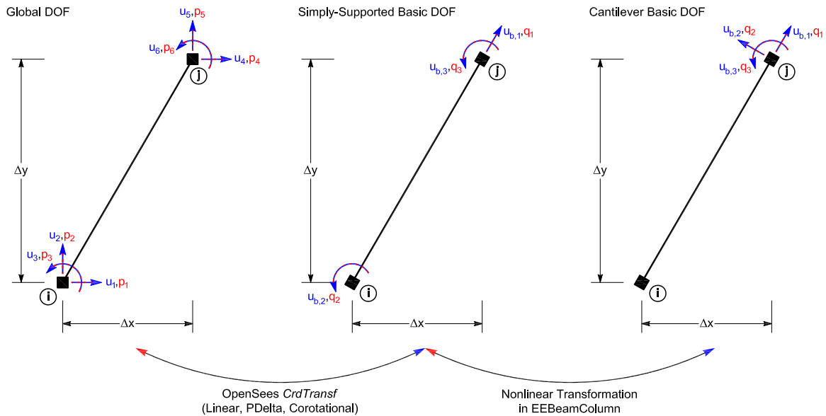
Fig. 6.22 Experimental beam-column element ( EEBeamColumn2d ).
