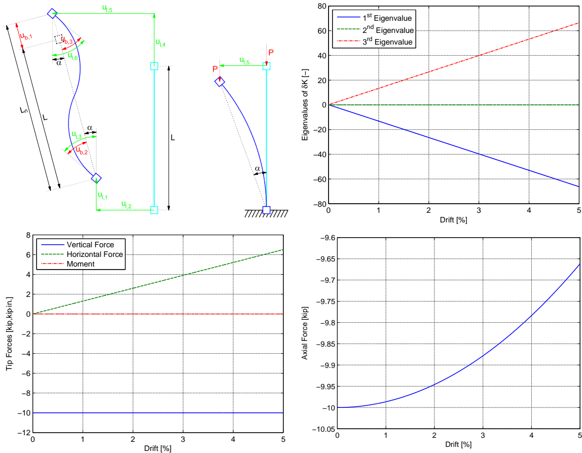
Fig. 4.18 Pushover analysis of elastic cantilever column with corotational geometric transformation: (a) geometry, (b) eigenvalues, (c) tip forces, (d) axial force.
