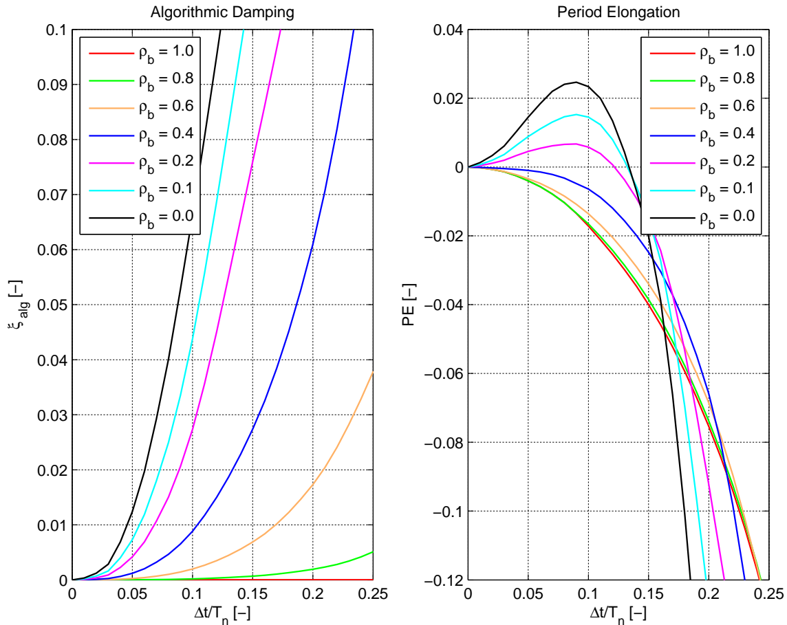
Fig. 4.28 Algorithmic damping ratios and relative period errors for explicit generalized-alpha (EG \alpha ) method.
