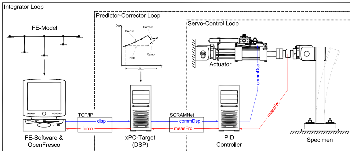
Fig. 5.4 Three-loop hardware architecture.
