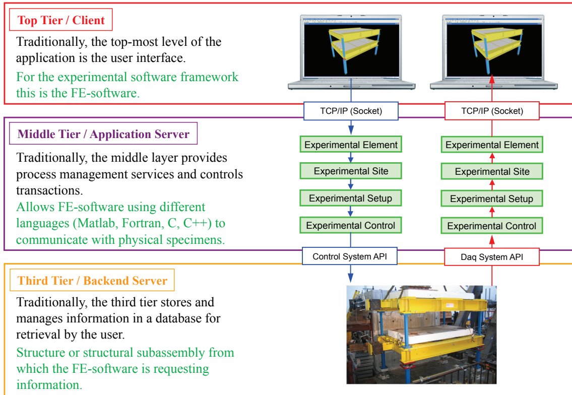
Fig. 3.3 Multi-tier software architecture.
