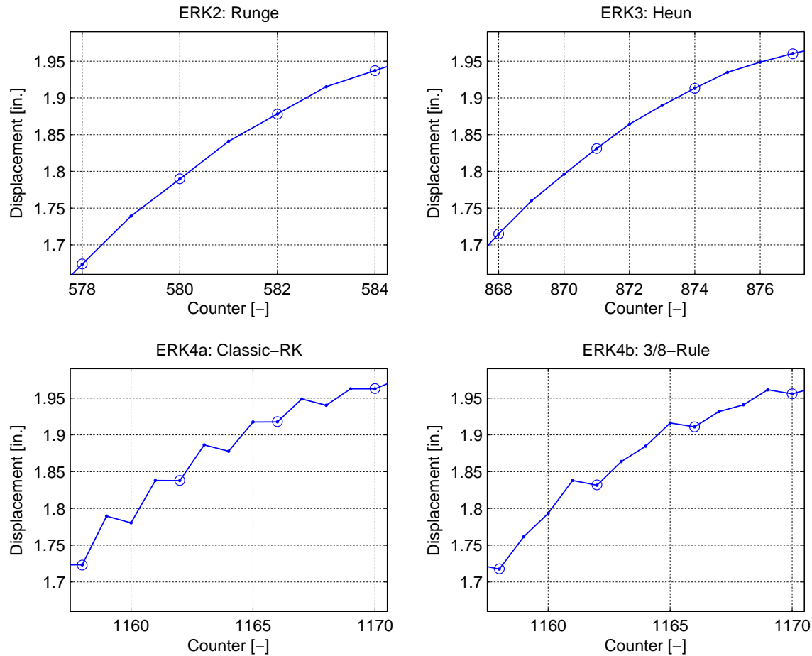
Fig. 4.30 ERK convergence comparison for one-bay-frame model.
