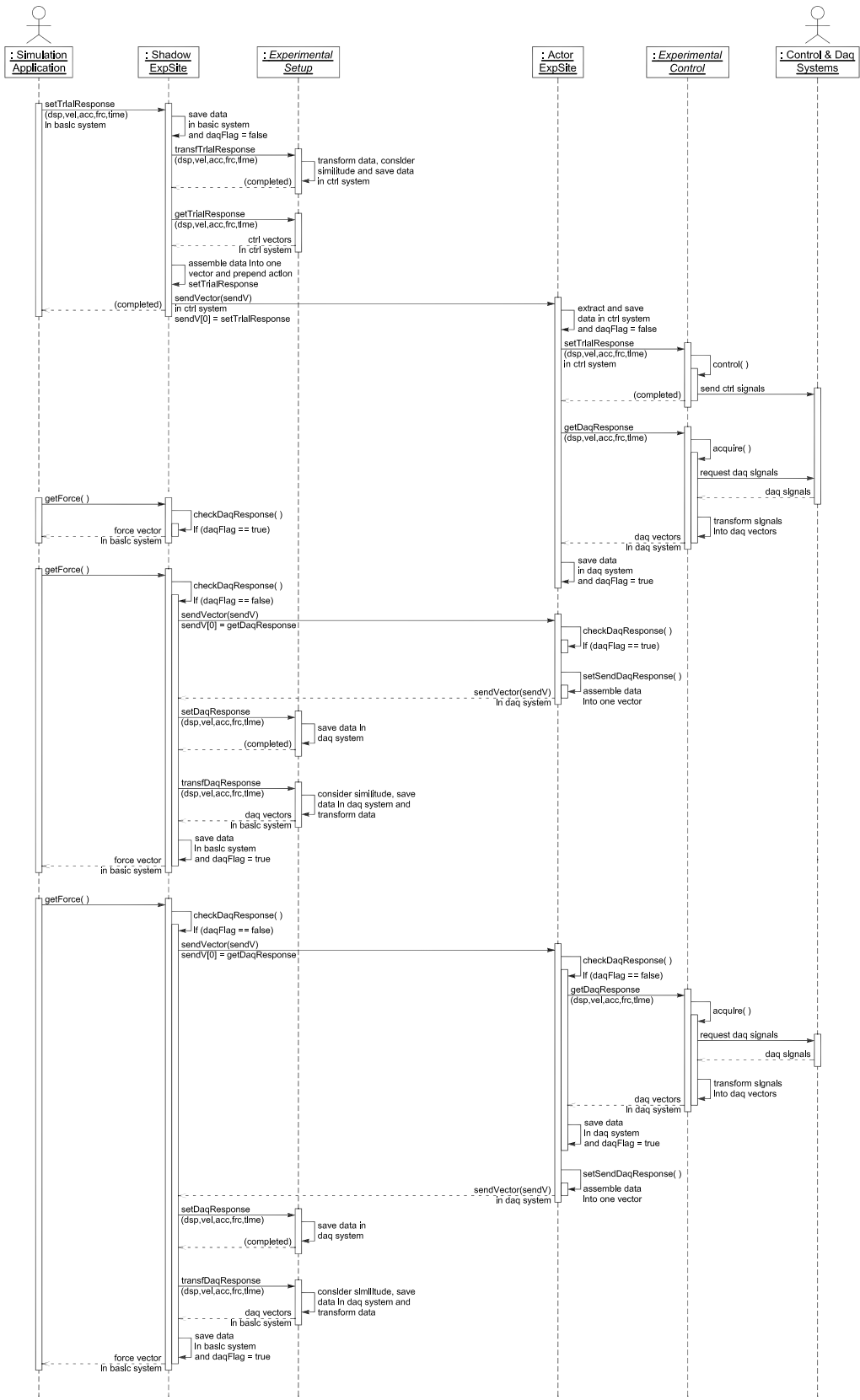
Fig. 3.14 OpenFresco sequence diagram for distributed deployment with ExperimentalSetup on computational client side.
