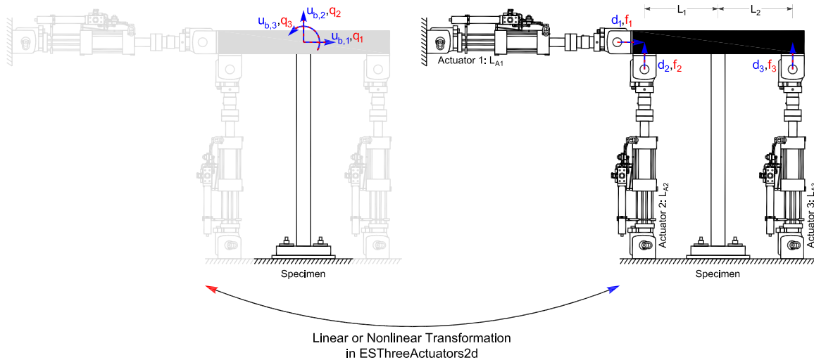
Fig. 3.25 Three actuators experimental setup (ESThreeActuators2d).
