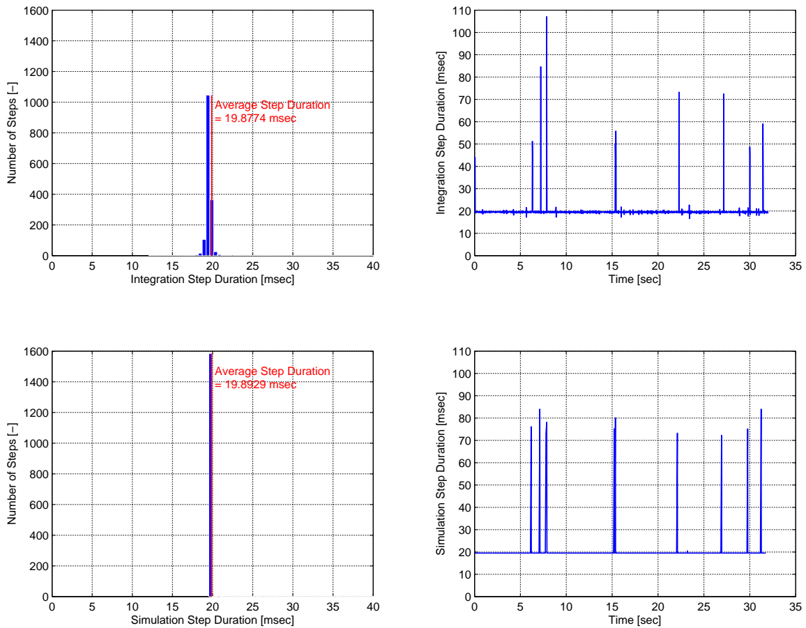
Fig. 6.8 Comparison of integration and simulation step distributions.
