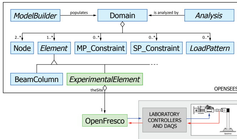
Fig. 3.31 OpenSees as the computational framework.
