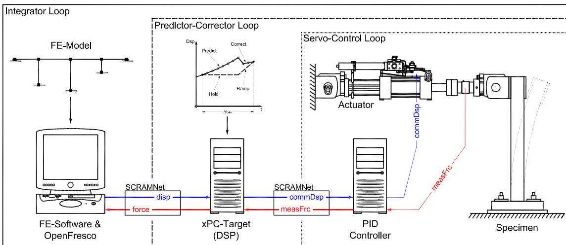
Fig. 3.29 SCRAMNet+ experimental control (ECSCRAMNet).
