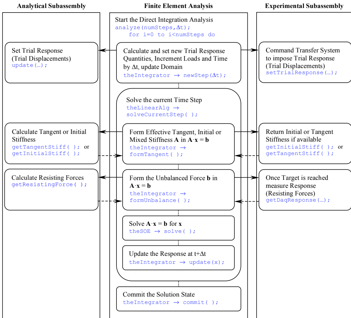
Fig. 2.2 Hybrid simulation testing procedure.
