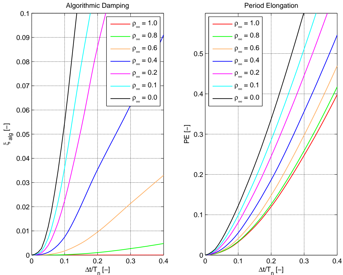
Fig. 4.29 Algorithmic damping ratios and relative period errors for implicit generalized-alpha (IG \alpha ) and generalized-alpha-OS (G \alpha OS) methods.
