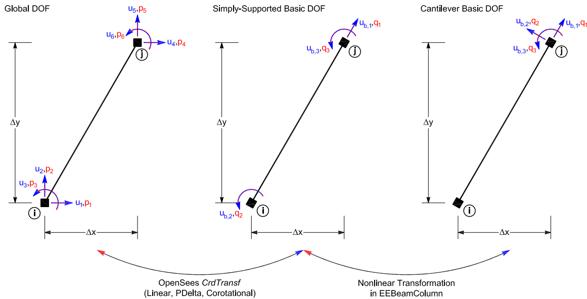
Fig. 3.16 Experimental beam-column element ( EEBeamColumn2d ).
