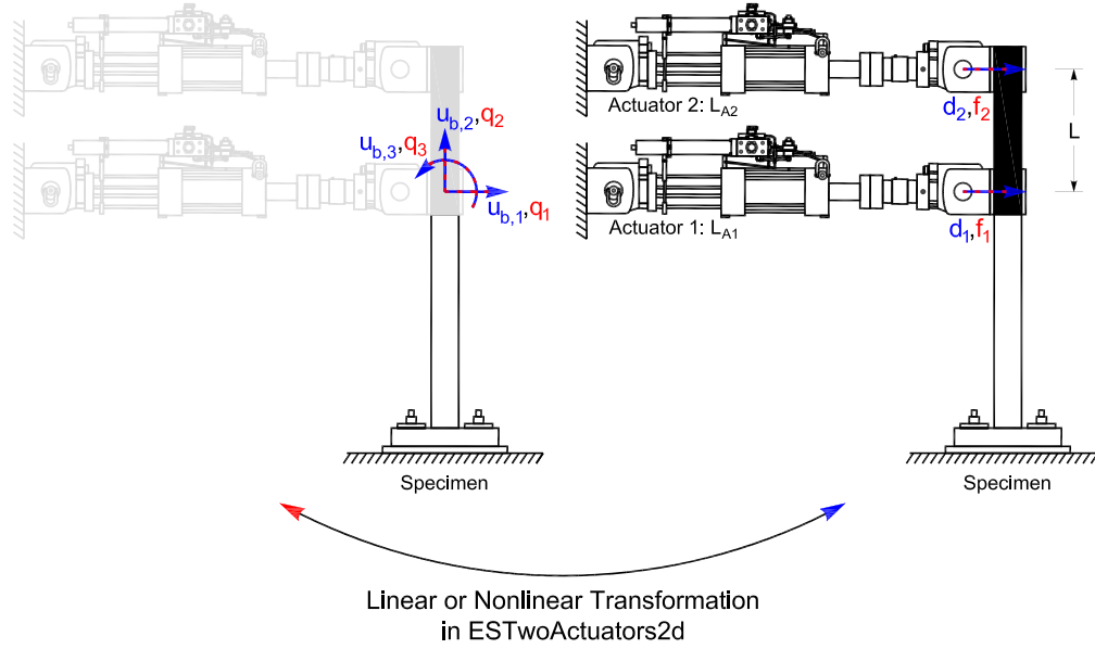
Fig. 3.24 Two actuators experimental setup (ESTwoActuators2d).
