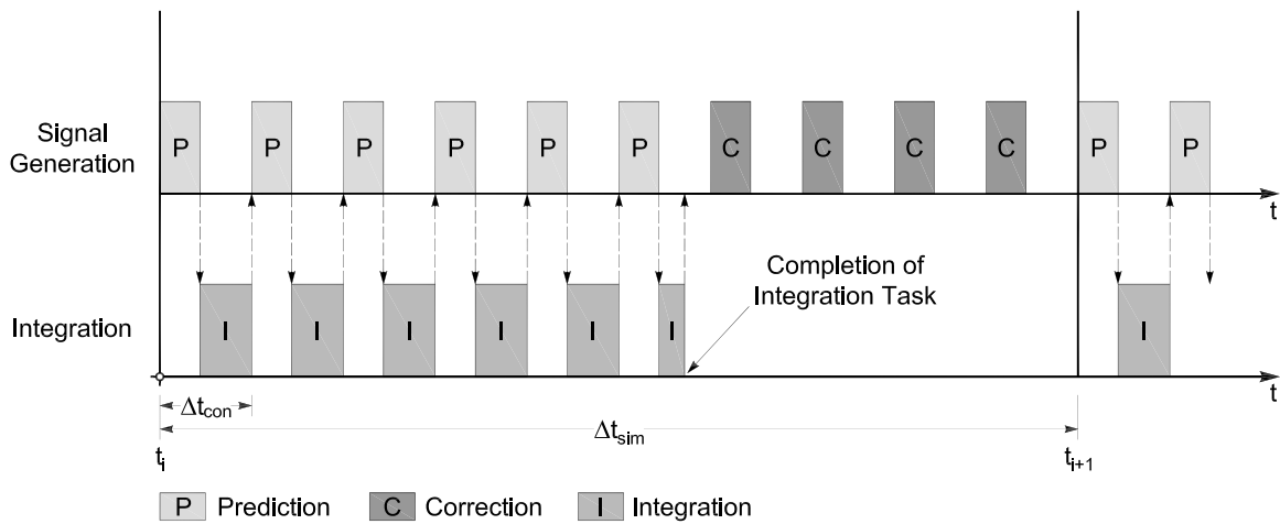
Fig. 5.2 Execution sequence in the case of one single digital signal processor.
