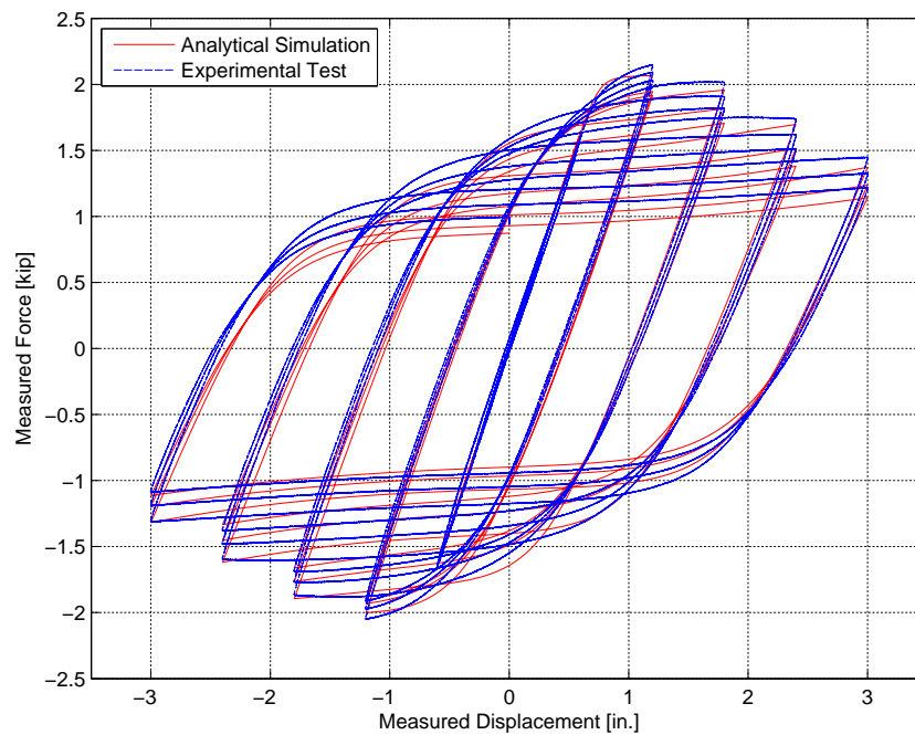
Fig. 6.19 Comparison of analytical versus experimental hysteresis loops for SAC loading history.
