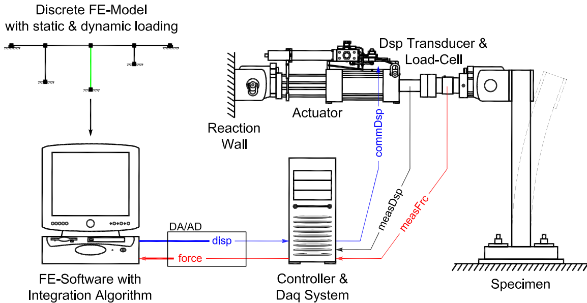
Fig. 2.1 Key components of a hybrid simulation.
