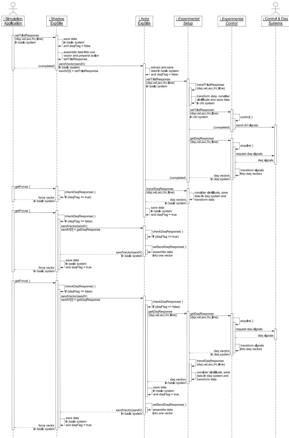
Fig. 3.13 OpenFresco sequence diagram for distributed deployment with xperimentalSetup on laboratory side.
