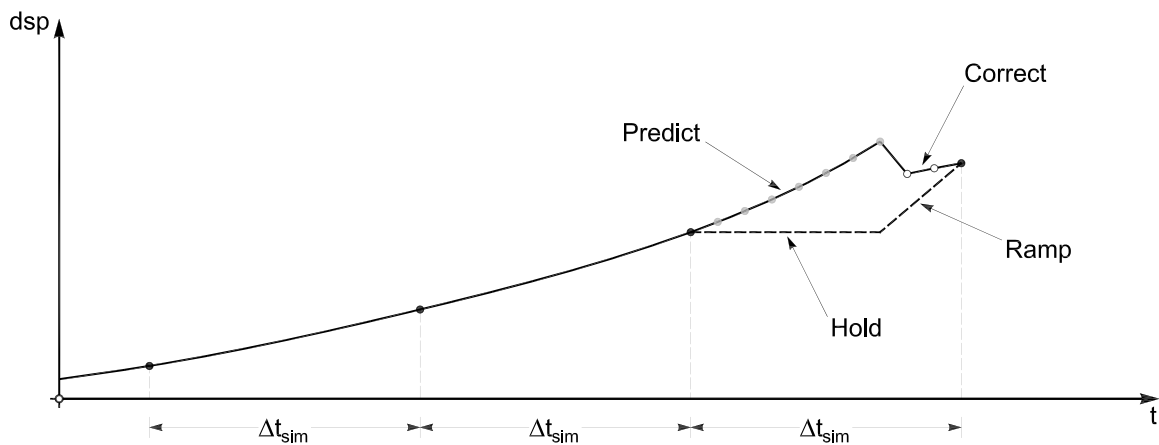
Fig. 5.1 Hold and ramp procedure vs. continuous testing procedure.
