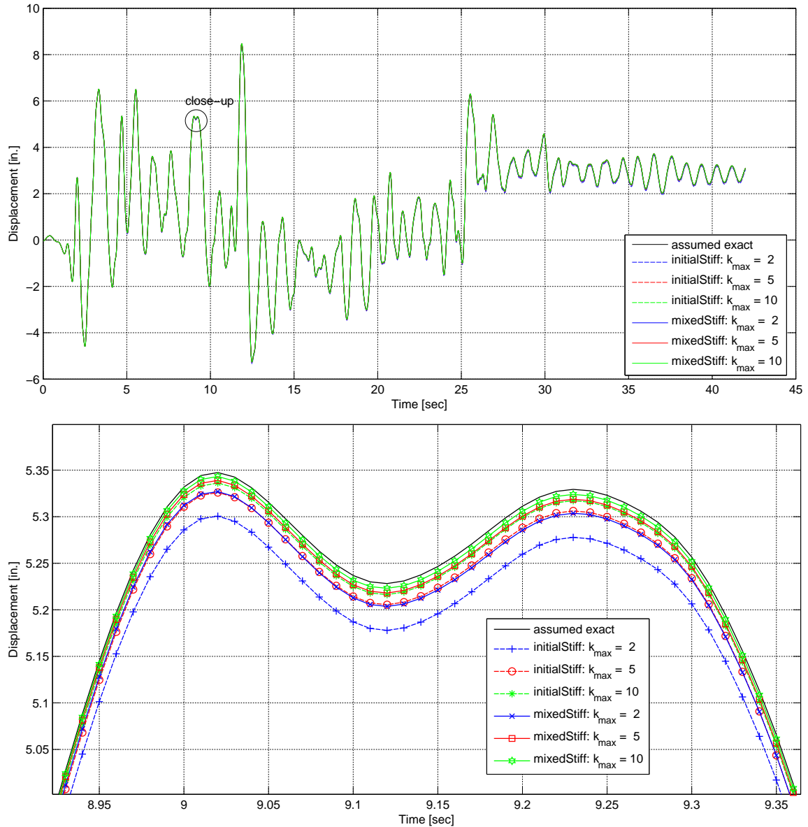
Fig. 4.12 Displacement comparison for four-story-frame model.
