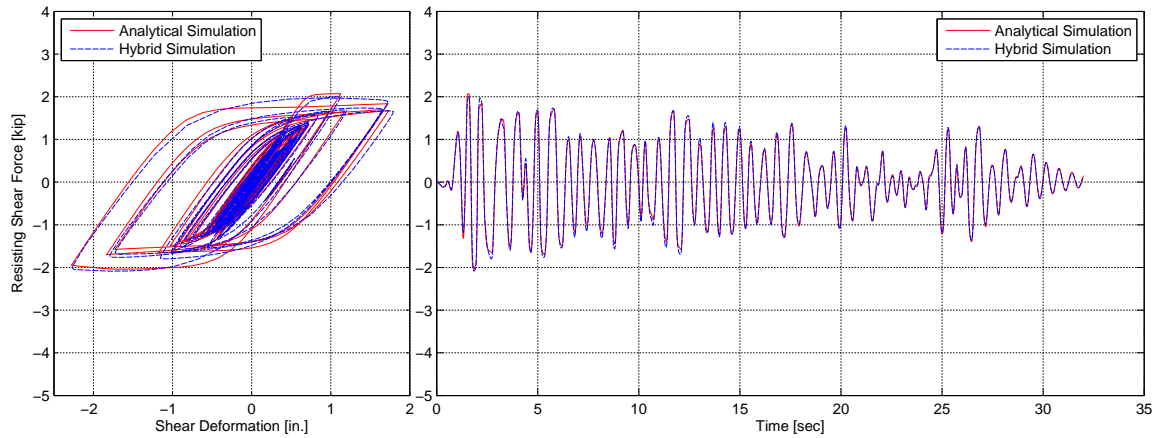
Fig. 6.21 Comparison of hysteresis loops and force histories of one-bay-frame model for analytical versus hybrid simulation.
