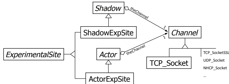
Fig. 3.22 Class diagram of client-server architecture.
