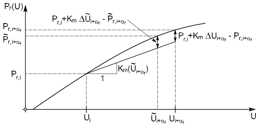
Fig. 4.19 Approximation of nonlinear resisting force using \mathbf{K}_m .
