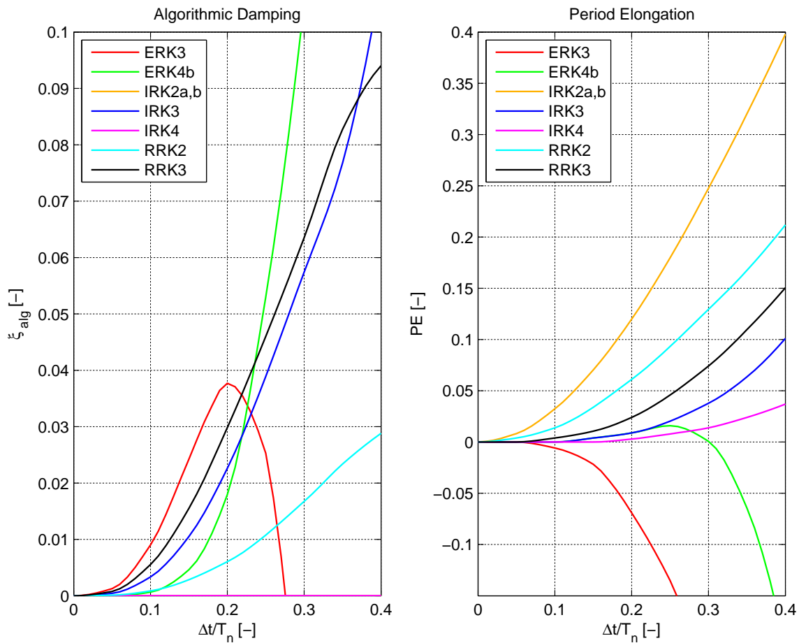
Fig. 4.39 Algorithmic damping ratios and relative period errors for Runge-Kutta methods.
