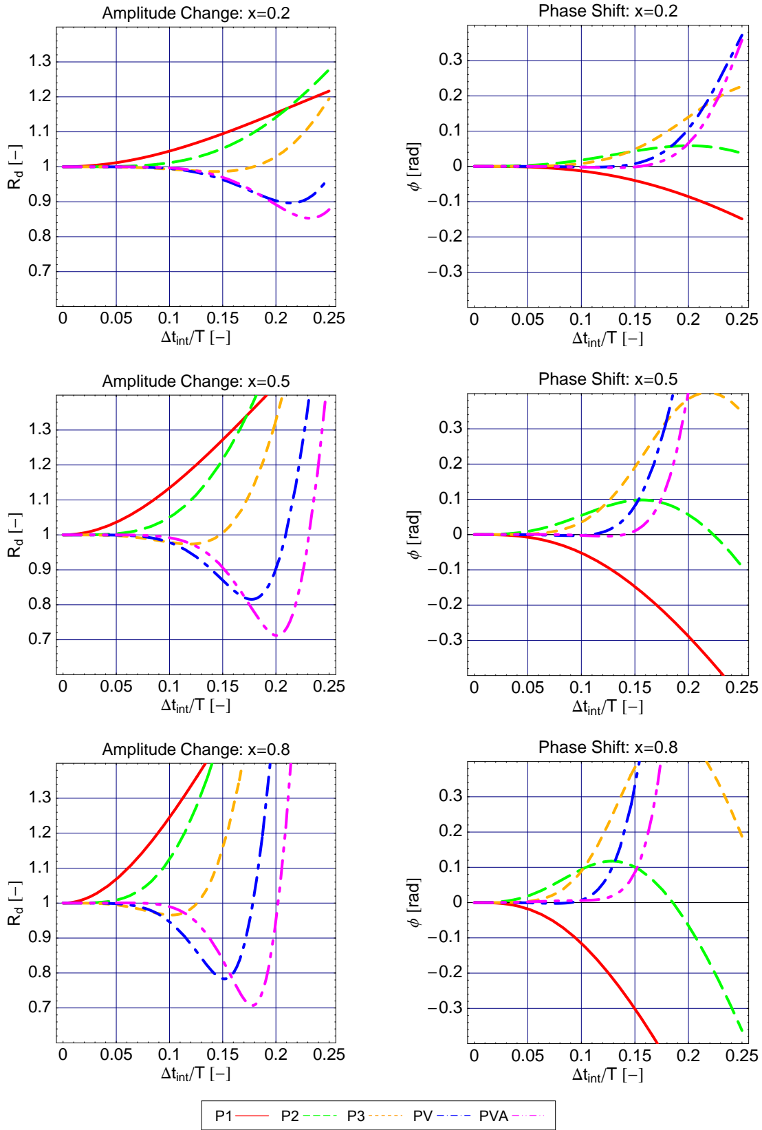
Fig. 5.12 Accuracies of predictors in terms of amplitude and phase.
