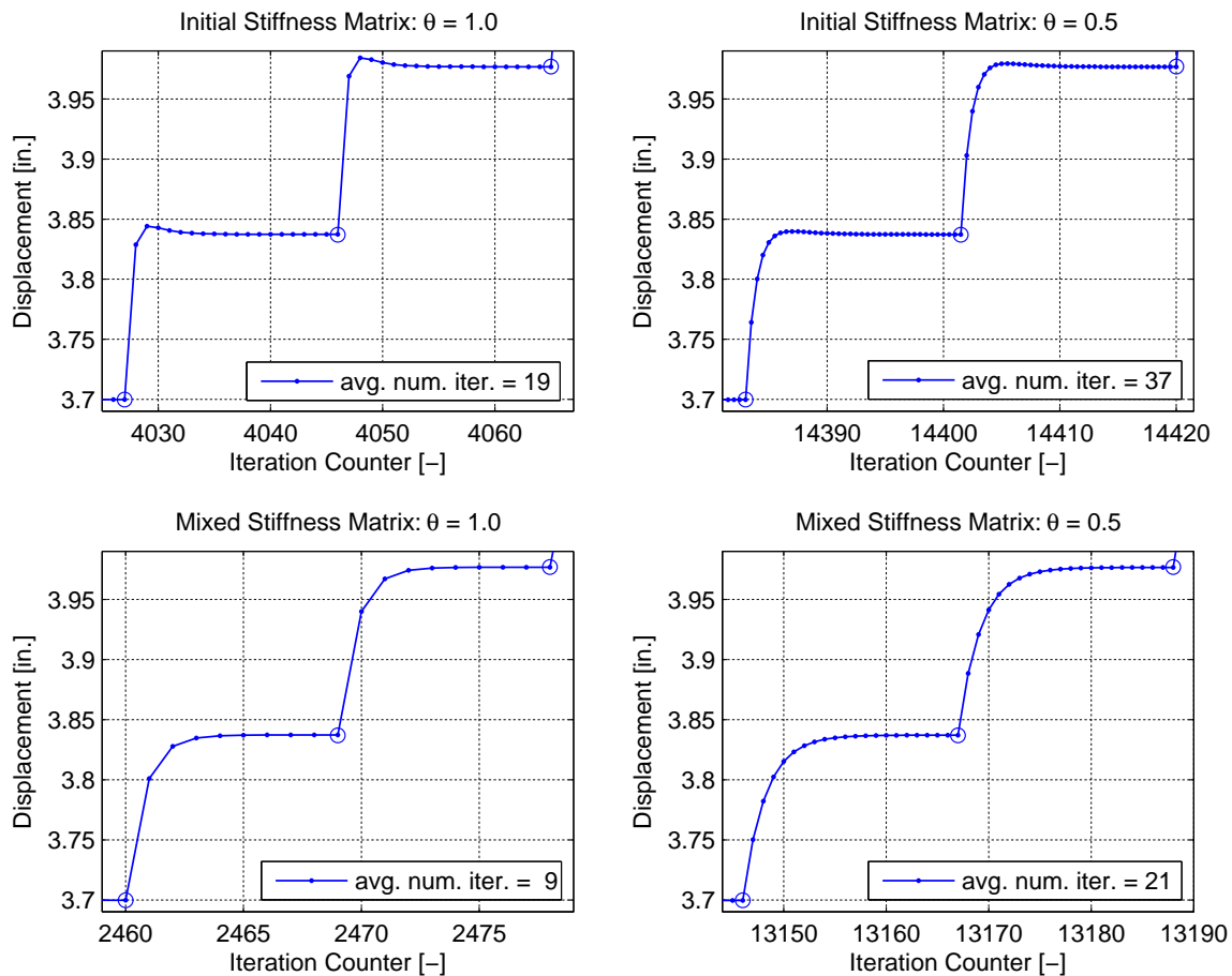
Fig. 4.8 Newton-Raphson convergence comparison for portal-frame model.
