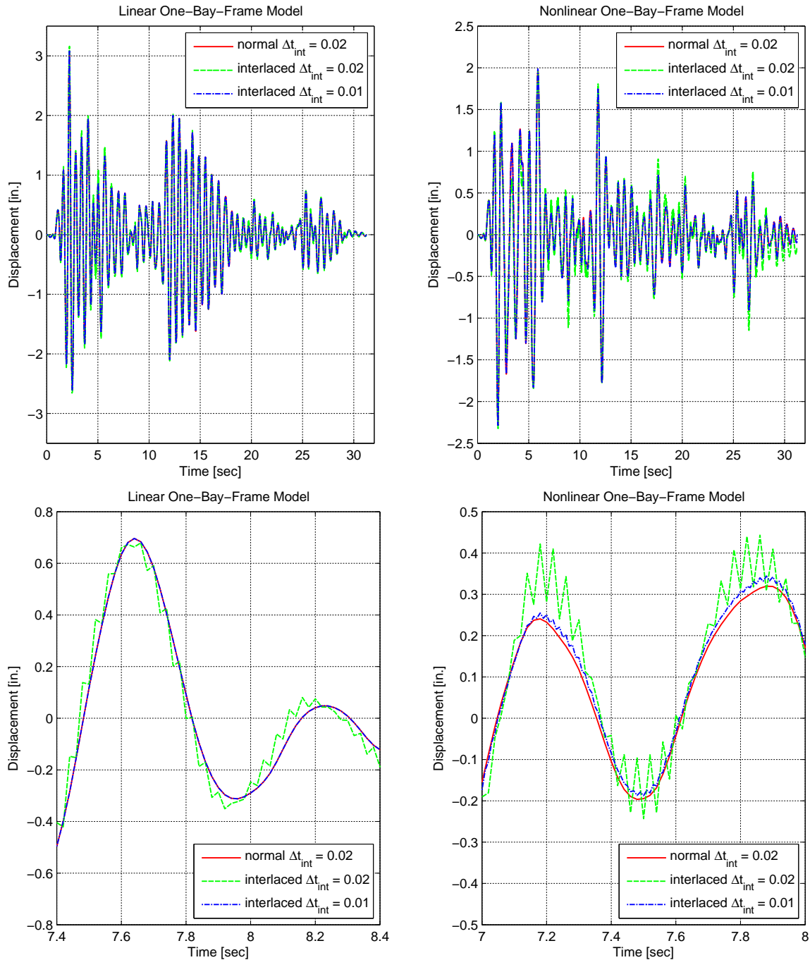
Fig. 5.18 Displacement command signal comparison for interlaced solution strategy.
