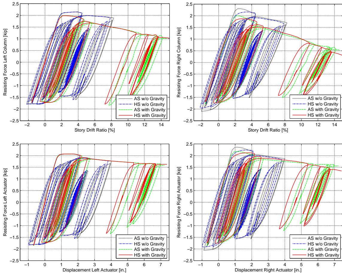
Fig. 6.33 Comparison of element force-story-drift and actuator force-displacement hysteresis loops of portal-frame model for analytical versus hybrid simulation.
