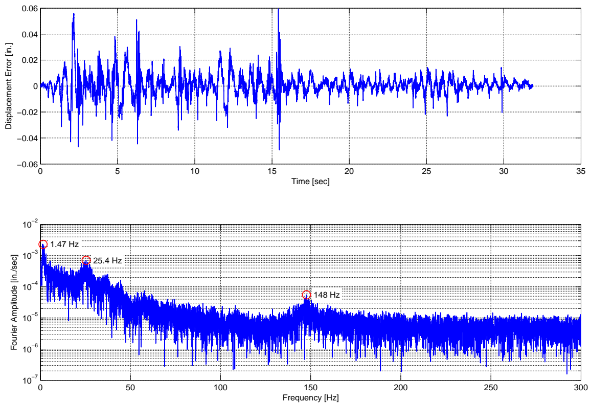
Fig. 6.12 Displacement error history and Fourier amplitude spectrum from STS.
