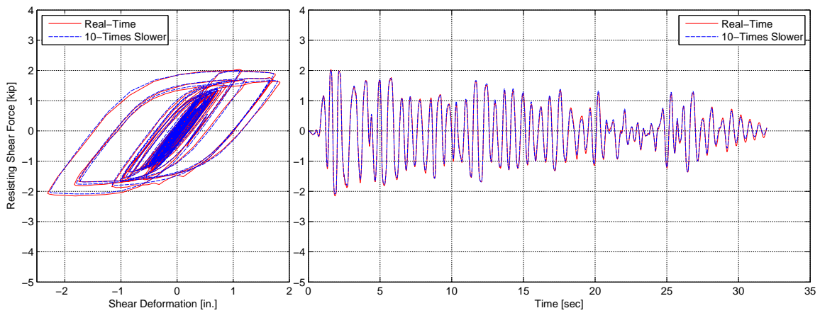
Fig. 6.16 Comparison of hysteresis loops and force histories of one-bay-frame model for real-time versus slow hybrid simulation.
