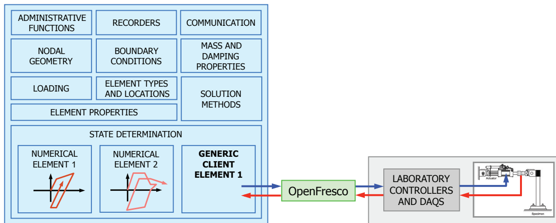
Fig. 3.1 Finite element analysis software of user’s choice, OpenFresco middleware, and physical specimen with control and data-acquisition systems in laboratory.
