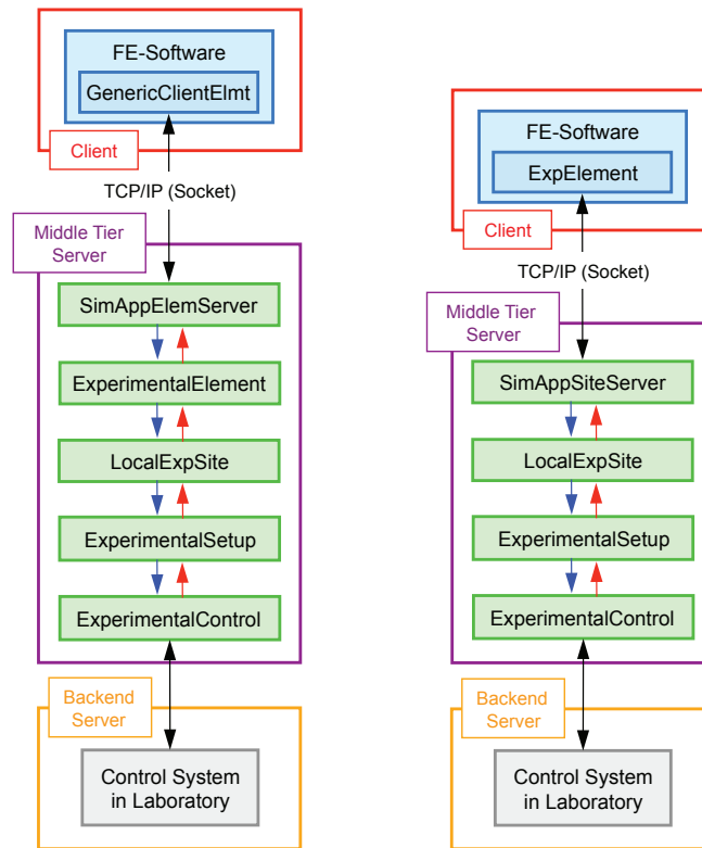
Fig. 3.4 Three-tier configurations for local deployment.
