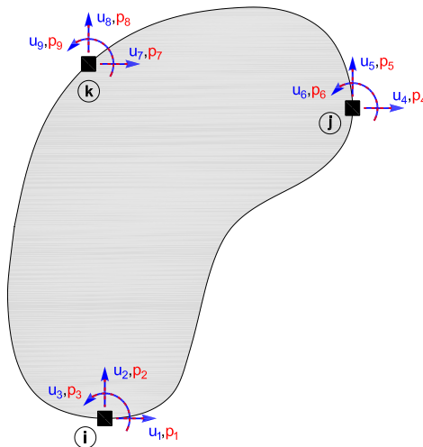
Fig. 3.20 Generic experimental element (EEGeneric).
