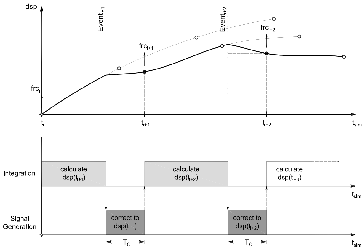
Fig. 5.20 Displacement path and execution sequence of constant correction-time strategy.
