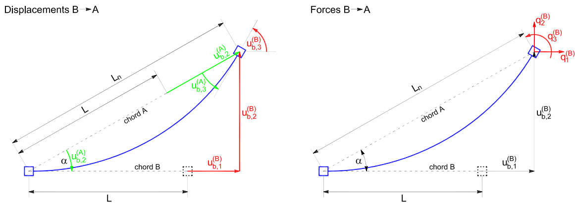
Fig. 3.18 Nonlinear transformations from basic system B to A.
