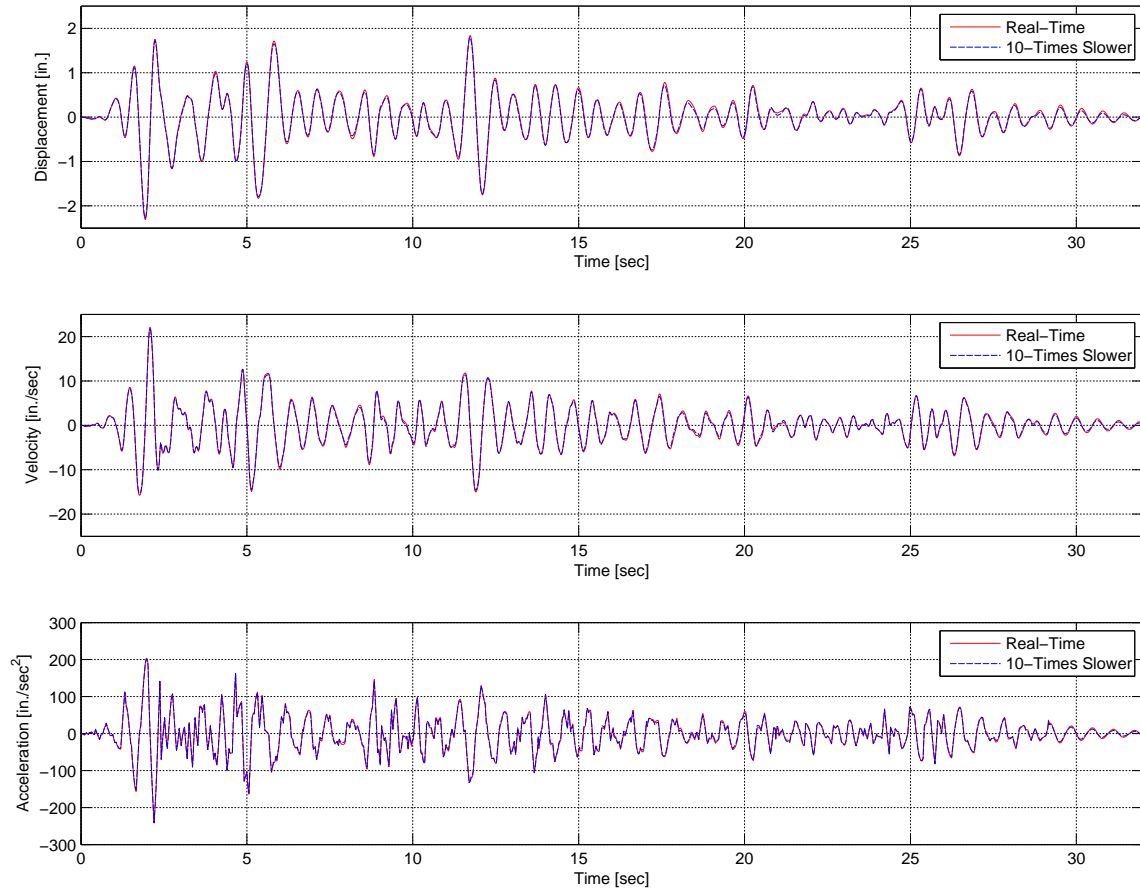
Fig. 6.15 Comparison of response histories of one-bay-frame model for real-time versus slow hybrid simulation.
