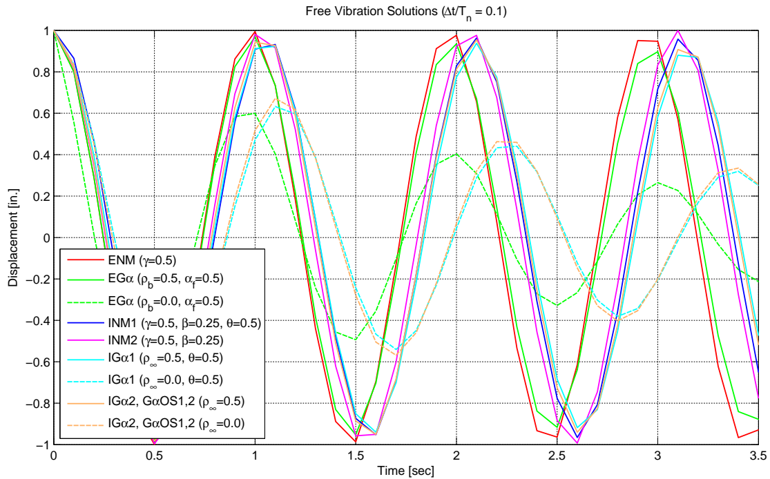
Fig. 4.23 Free vibration solutions for direct integration methods.
