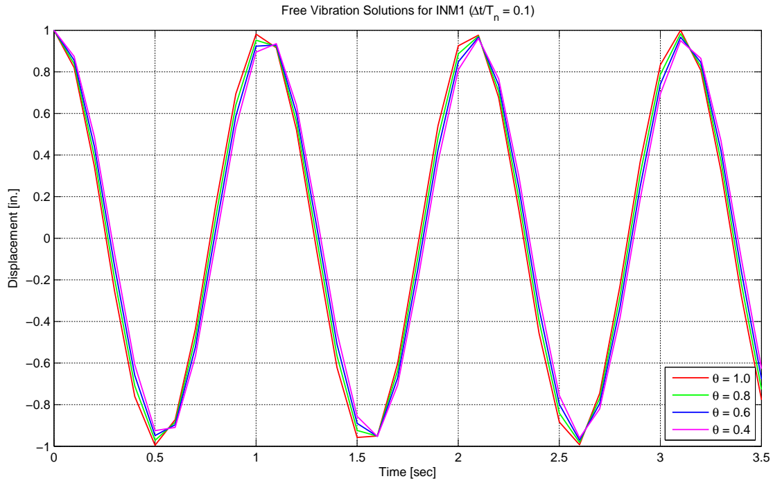
Fig. 4.25 Free vibration solutions for implicit Newmark (INM1) method.
