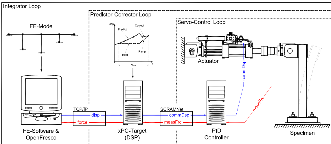
Fig. 3.28 xPC Target experimental control (ECxPCtarget).
