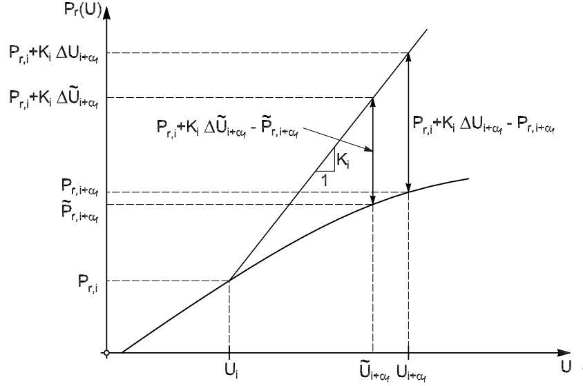
Fig. 4.16 Approximation of nonlinear resisting force using \mathbf{K}_i .
