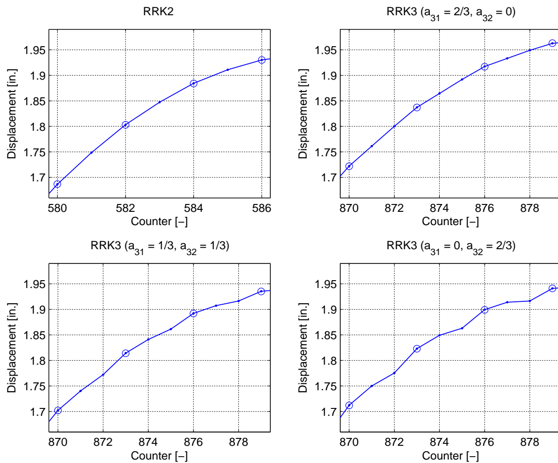
Fig. 4.35 RRK convergence comparison for one-bay-frame model.
