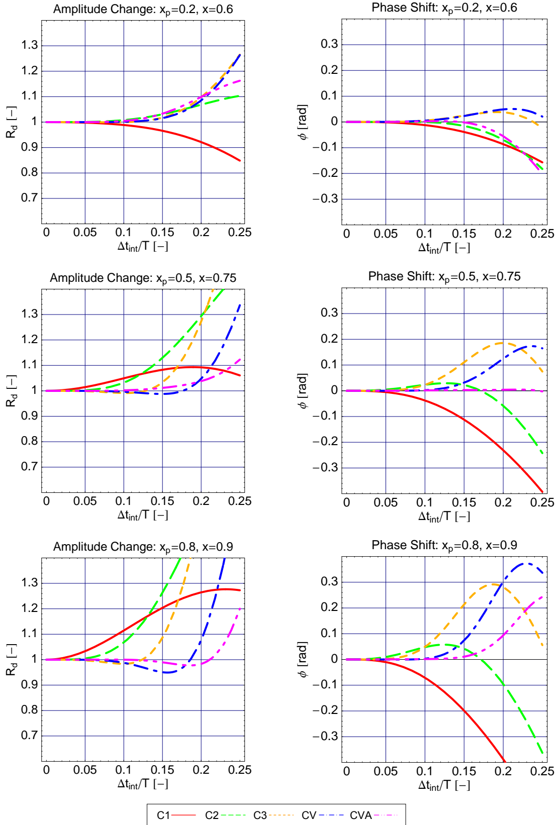
Fig. 5.14 Accuracies of correctors including last predicted displacement.
