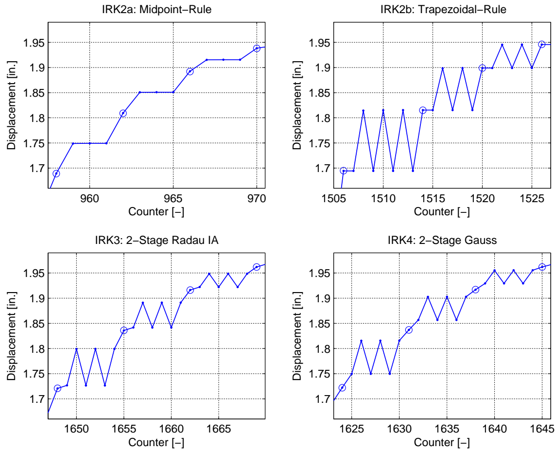
Fig. 4.33 IRK convergence comparison for one-bay-frame model.
