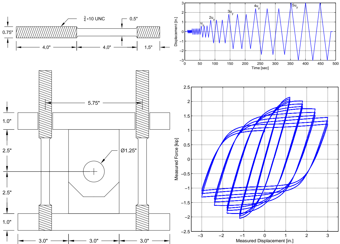
Fig. 6.4 Connection with coupon details and displacement history with hysteresis loops.
