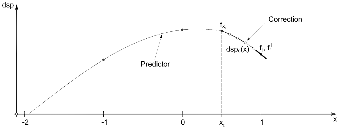
Fig. 5.9 Corrector using a second-order polynomial including the last predicted value.
