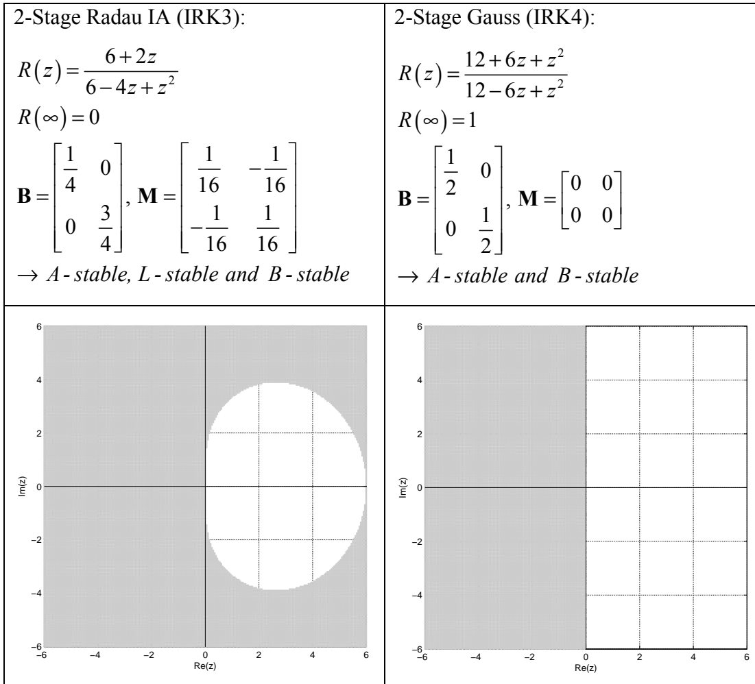
Fig. 4.37 Regions of Absolute Stability (RAS) for IRK methods.
