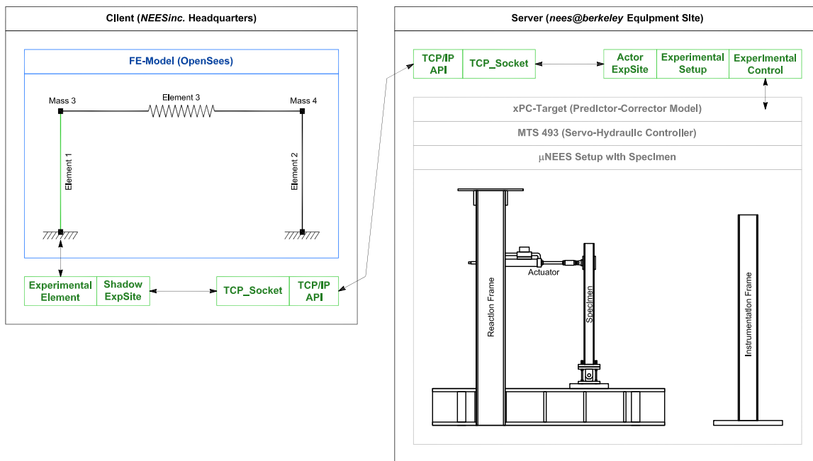
Fig. 6.5 Client-server configuration.
