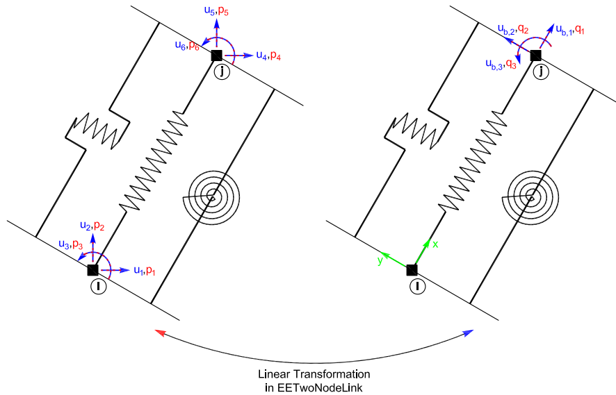
Fig. 3.19 Experimental two-node link element (EETwoNodeLink).
