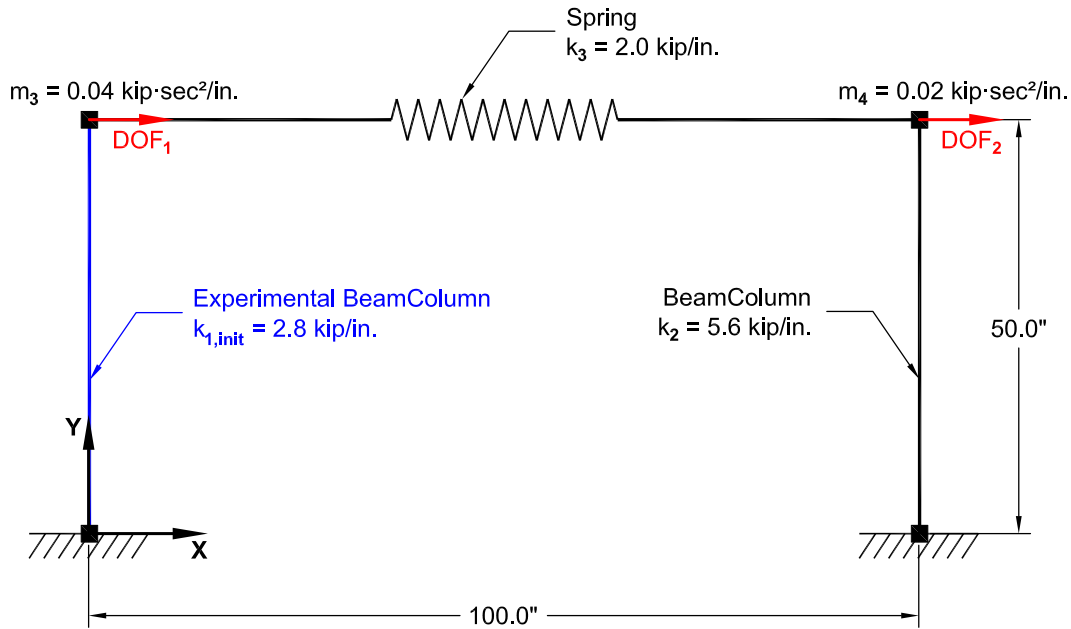
Fig. 6.1 One-bay-frame model with structural properties.
