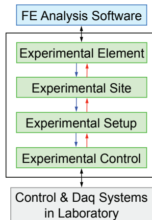
Fig. 3.2 Abstract components of the OpenFresco software architecture.
