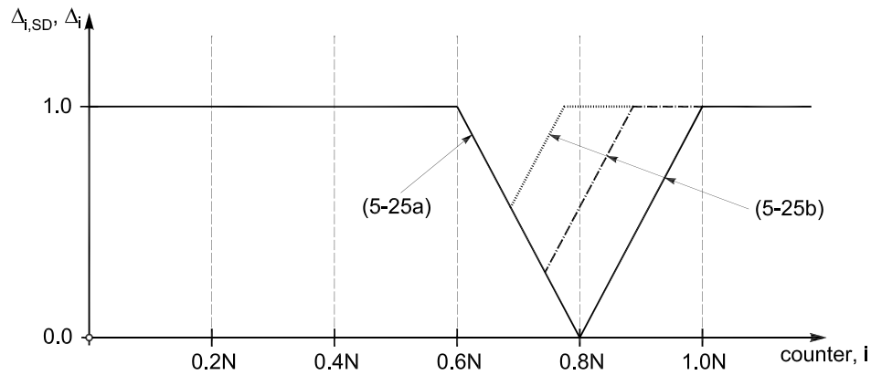
Fig. 5.16 Relationship between counter-increment and counter for smooth velocity transitions.
