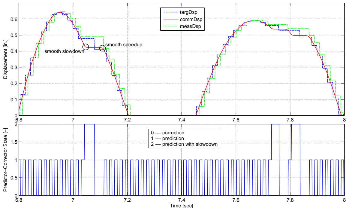
Fig. 6.11 Close up of predictor-corrector state transitions from xPC Target.
