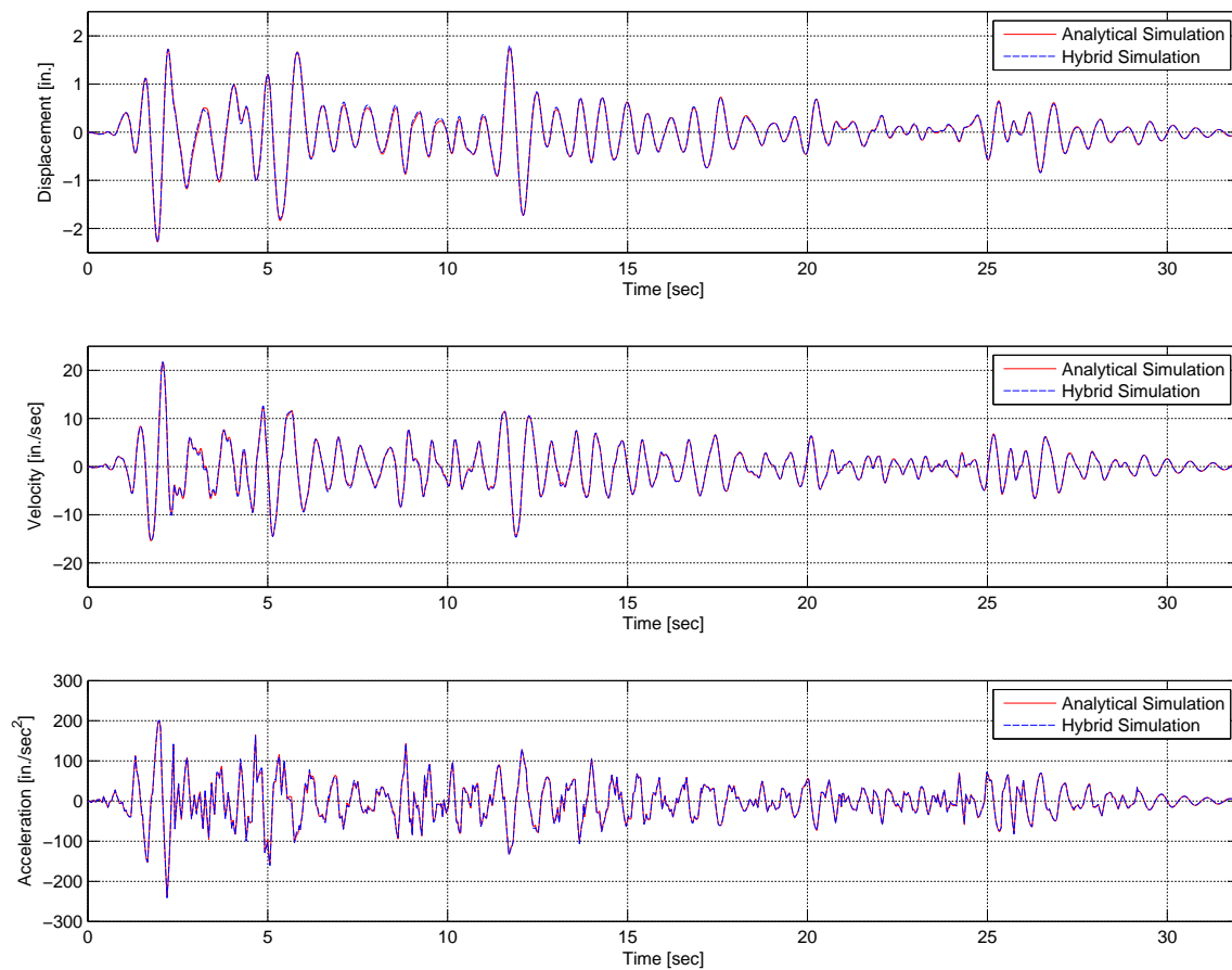
Fig. 6.20 Comparison of response histories of one-bay-frame model for analytical versus hybrid simulation.
