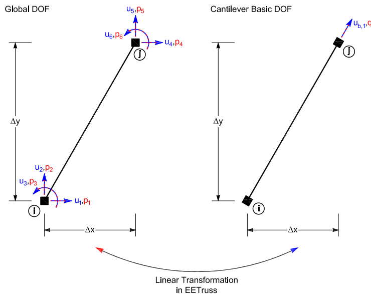
Fig. 3.15 Experimental truss element (EETruss).
