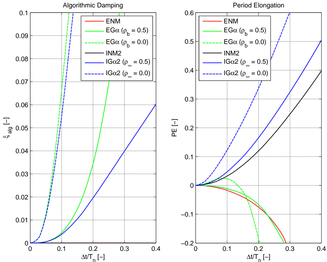
Fig. 4.27 Algorithmic damping ratios and relative period errors for direct integration methods.
