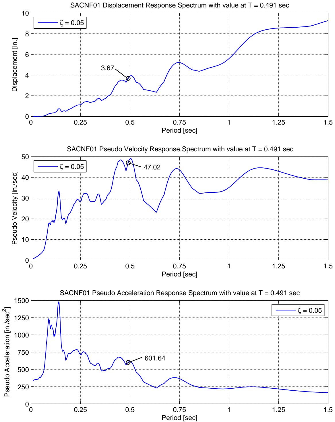
Fig. 6.25 Elastic response spectra for SACNF01 ground motion, with values at fundamental period.
