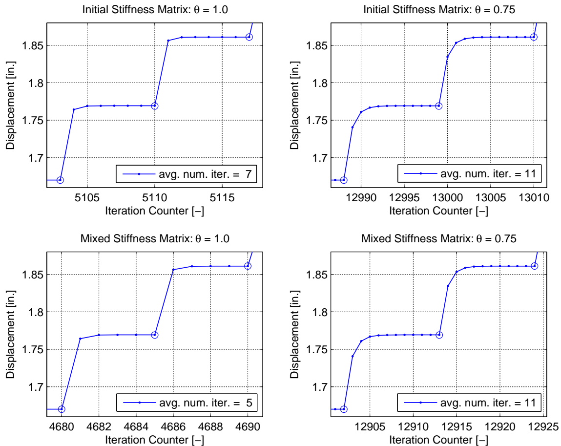
Fig. 4.6 Newton-Raphson convergence comparison for four-story-frame model.
