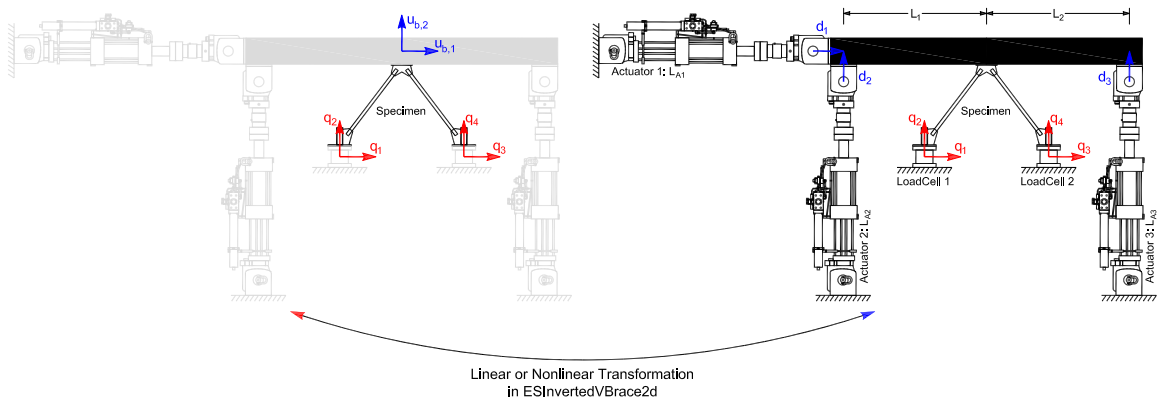
Fig. 3.26 Inverted-V brace experimental setup (ESInvertedVBrace2d).
