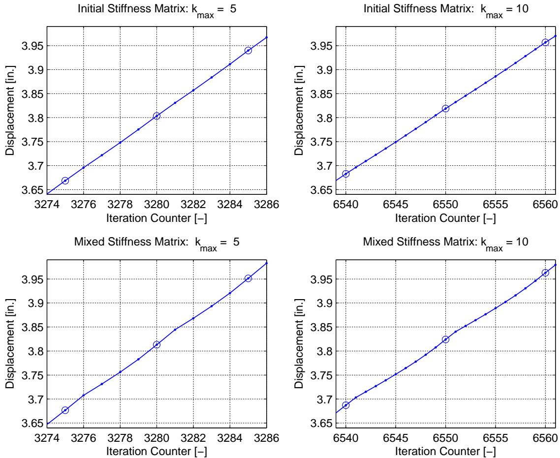
Fig. 4.13 Convergence comparison for portal-frame model.
