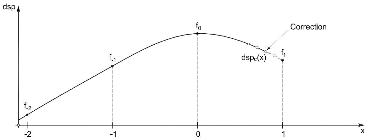
Fig. 5.6 Corrector using a third-order Lagrange polynomial.
