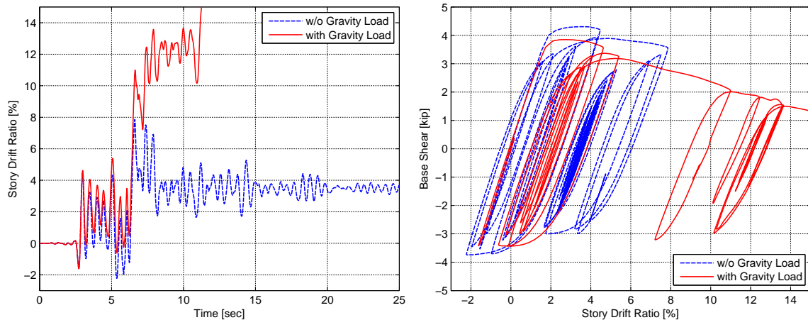
Fig. 6.26 Comparison of story-drift time-histories and total story hysteresis loops for portal-frame model from OpenSees.
