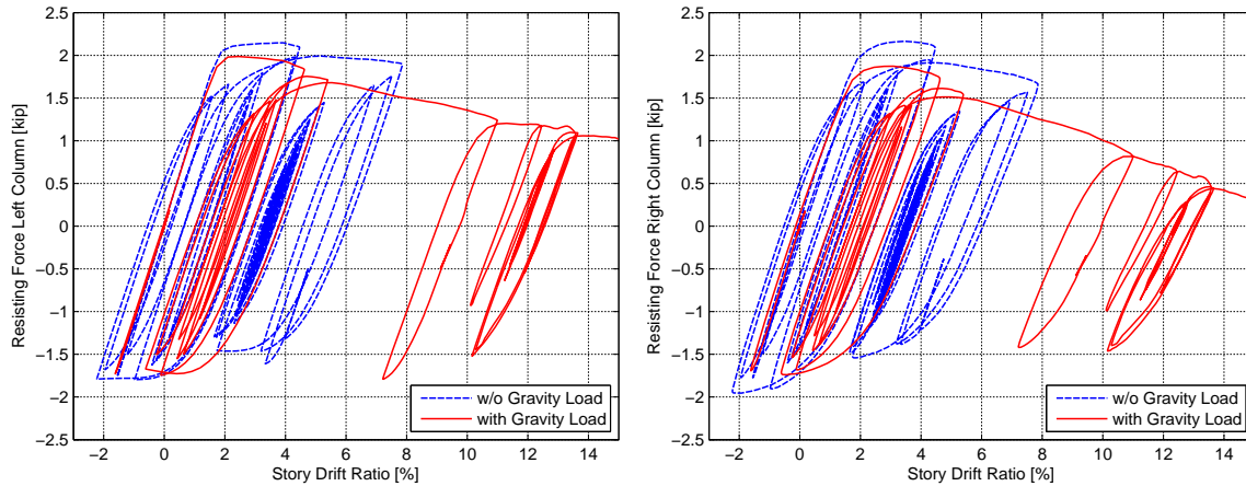
Fig. 6.27 Comparison of element force-story-drift hysteresis loops for portal-frame model from OpenSees.
