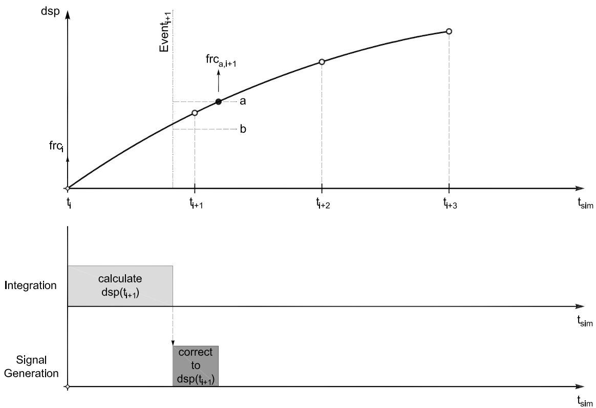
Fig. 5.19 Difficulties with solution strategy that is skipping head.
