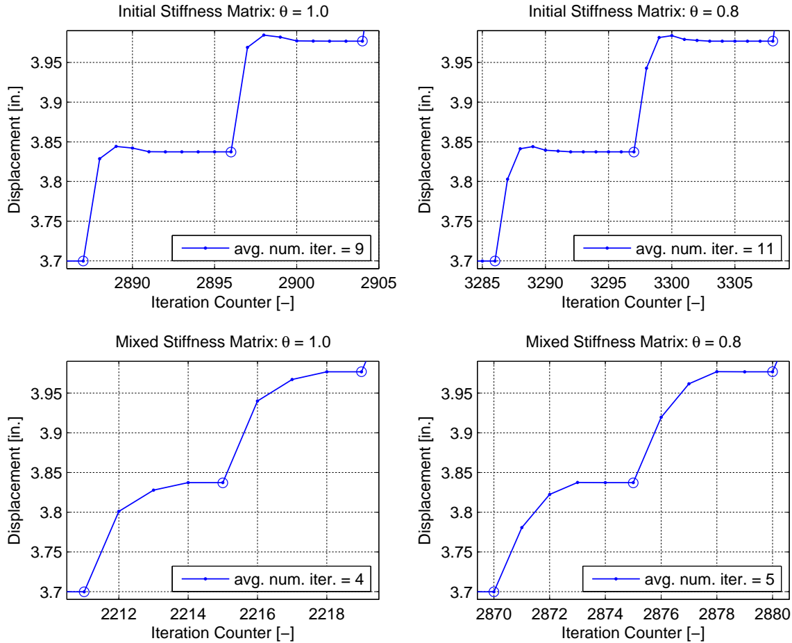
Fig. 4.9 Krylov-Newton convergence comparison for portal-frame model.
