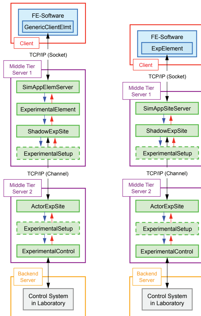
Fig. 3.5 Four-tier configurations for network deployment.
