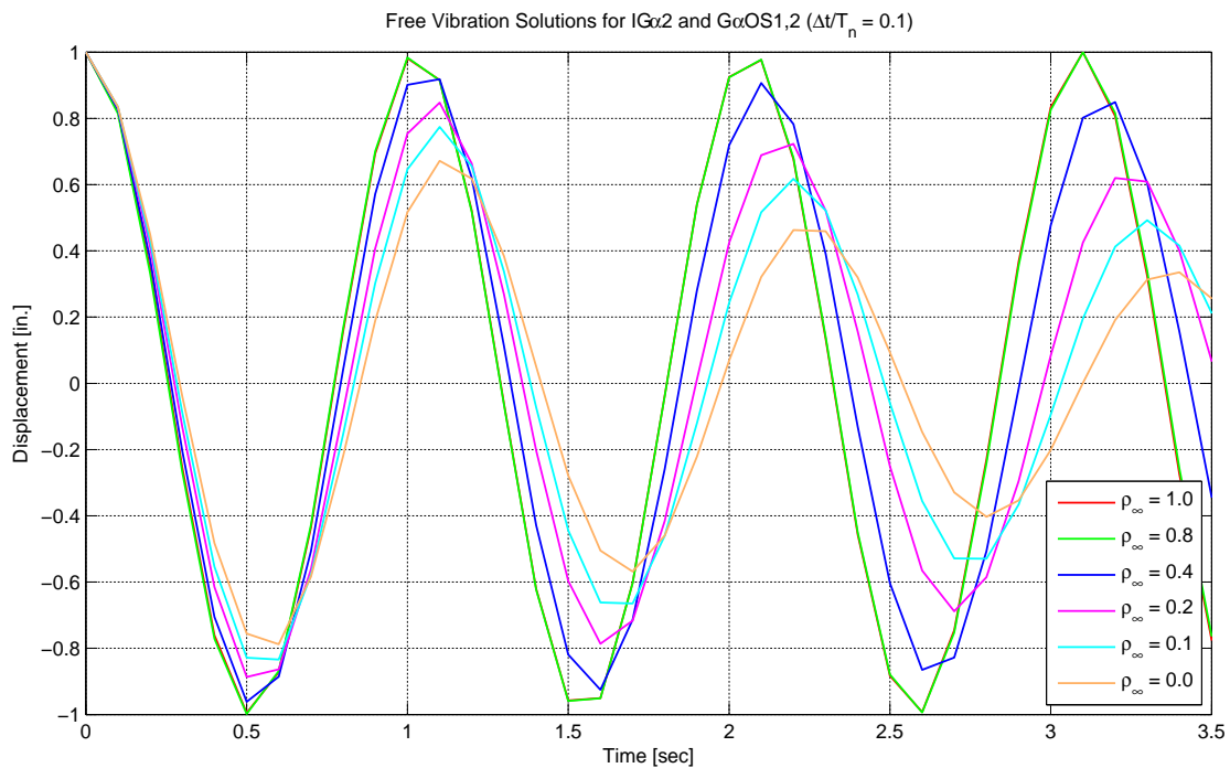
Fig. 4.26 Free vibration solutions for implicit generalized-alpha (IGα2) method.
