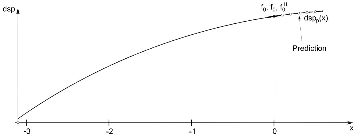
Fig. 5.10 Constant acceleration predictor.
