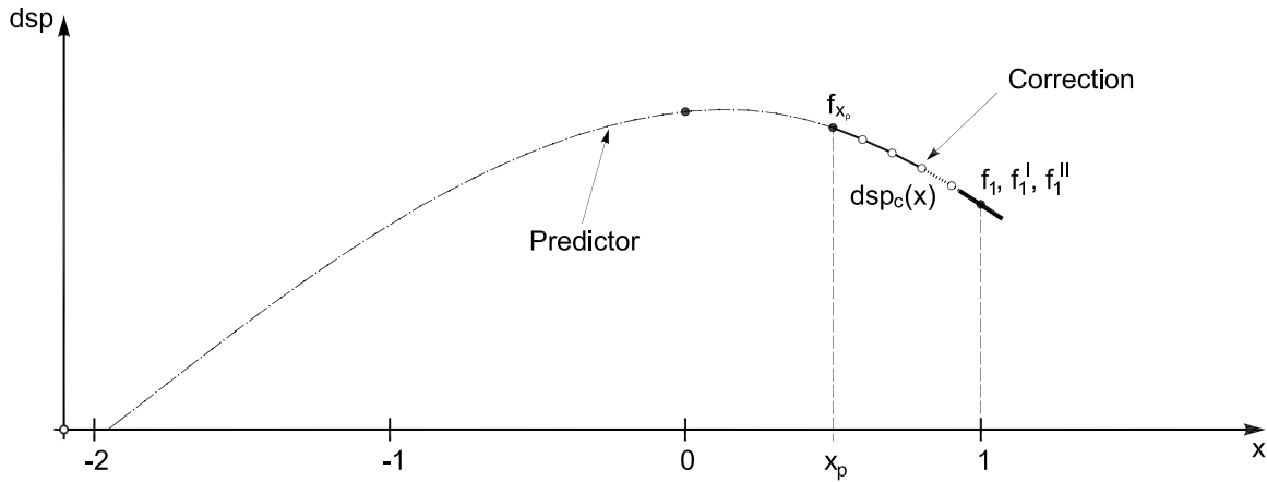
Fig. 5.11 Corrector using a third-order polynomial including the last predicted value.
